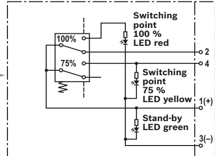
WE-2SP-M12x1
