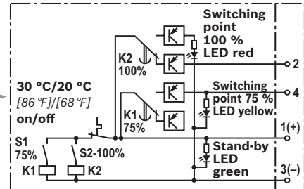
WE-2SPSU-M12x1
