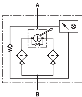
Duplex filter with bypass and mechanical indicator
