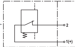
WE-1SP-EN175301-803
