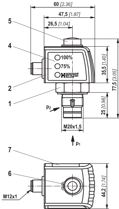
Pressure differential indicator with assembled switching element M12x1
