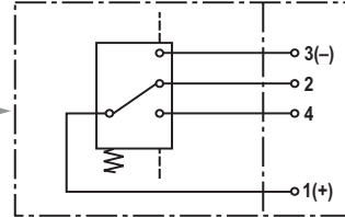
WE-1SP-M12x1
